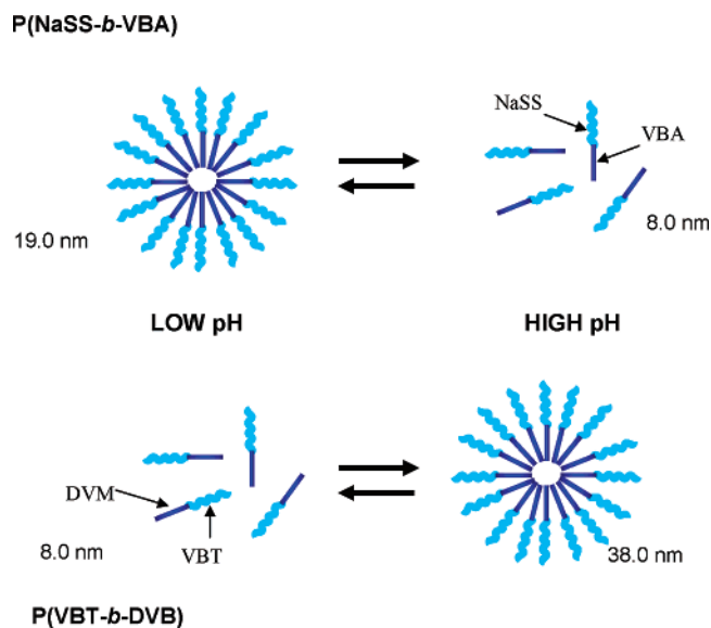
FIGURE 4. Schematic representation of AB diblock aggregation with changes in solution pH.
